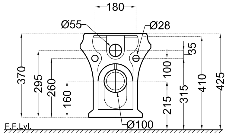
BACK VIEW
