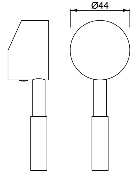
HANDLE
