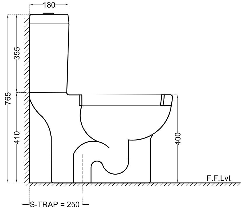
SIDE VIEW
